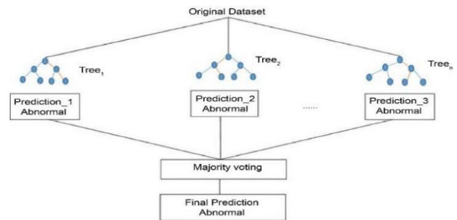
Fig. 7. Random Forest Classifier Architecture (3).
