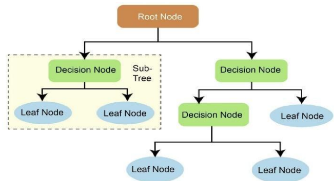
Fig. 8. Decision Tree Architecture (4).
