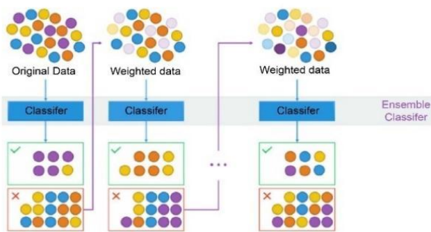
Fig. 5. Adaboosting Model Architecture (1).
