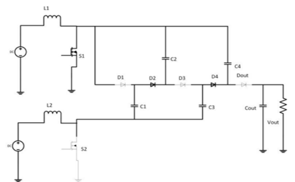
Fig.6. Mode 3 of Multiport Converter
