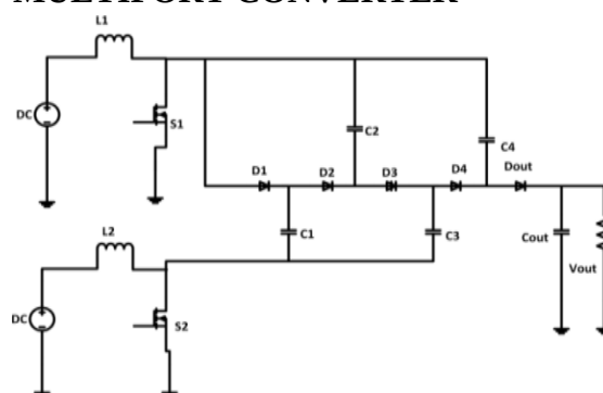
Fig.3 Proposed Multiport Converter
