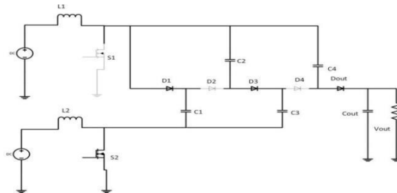
Fig.5 Mode 2 of Multiport Converter
