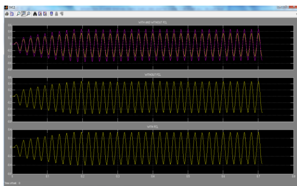
Fig.13. With and Without SFCL Voltage and Current
