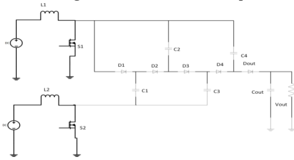
Fig.4. Mode 1 of Multiport Converter
