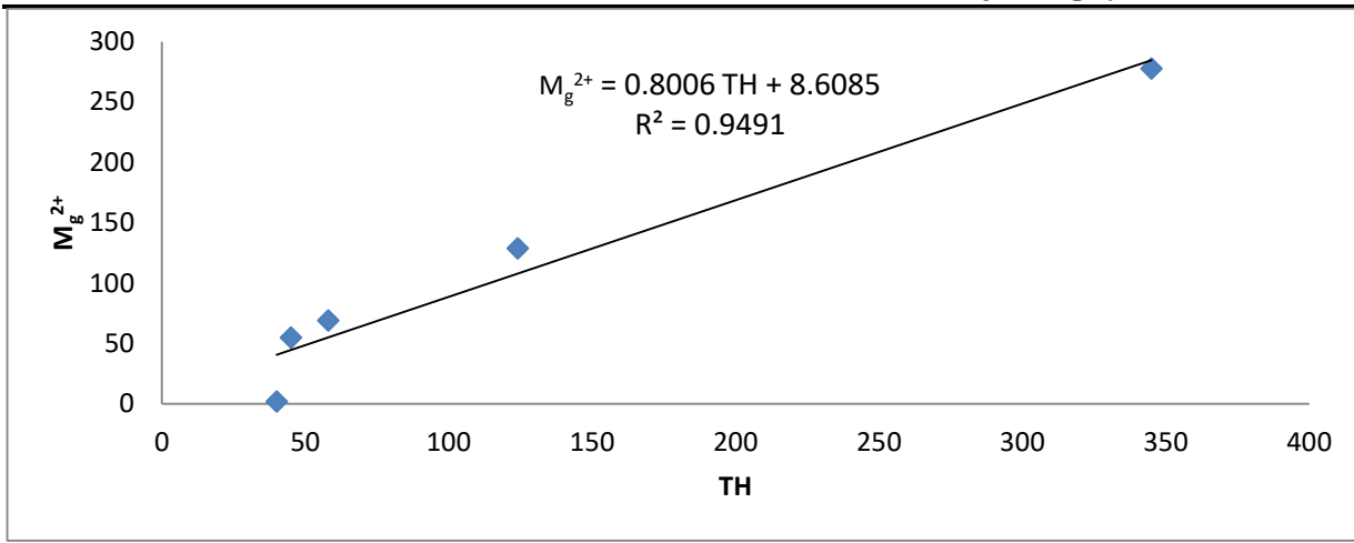
Fig 11: Correlation between TH and Mg^{2+}
