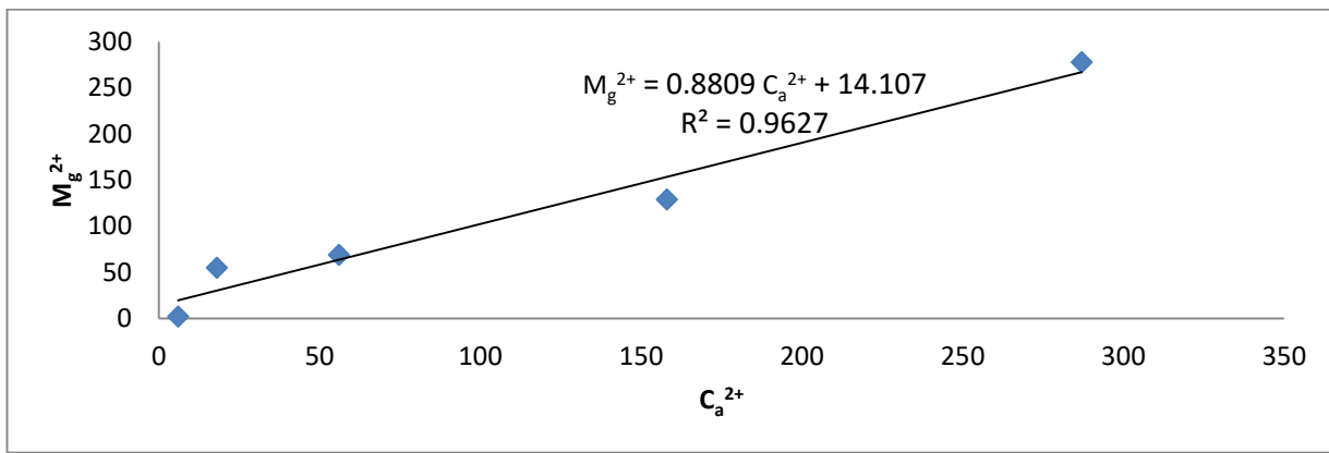
Fig 12: Correlation between Ca^{2+} and Mg^{2+}
