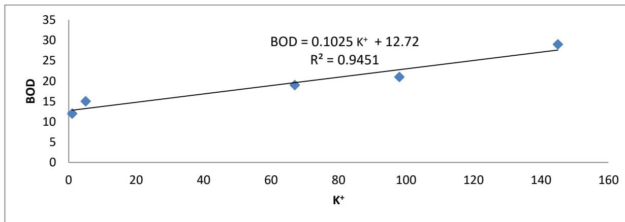
Fig 18: Correlation between K + and BOD
