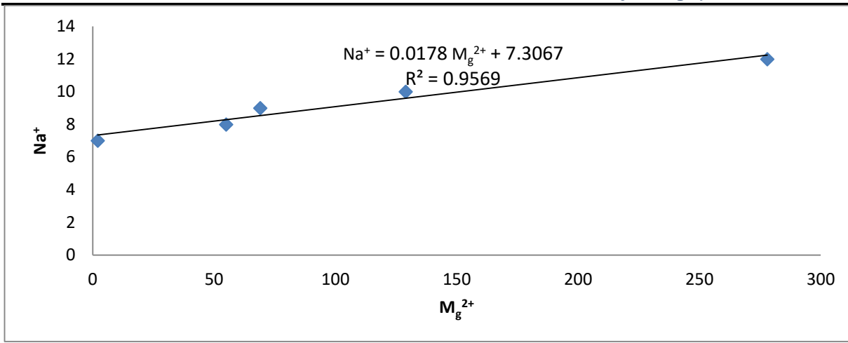
Fig 14: Correlation between M g 2+ and Na +
