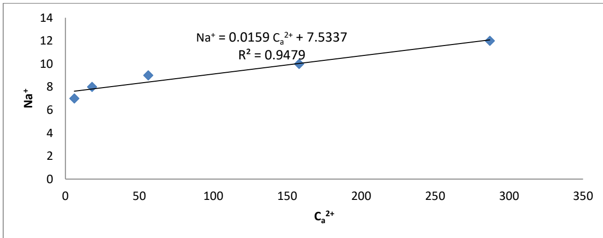
Fig 13: Correlation between Ca^{2+} and Na^+
