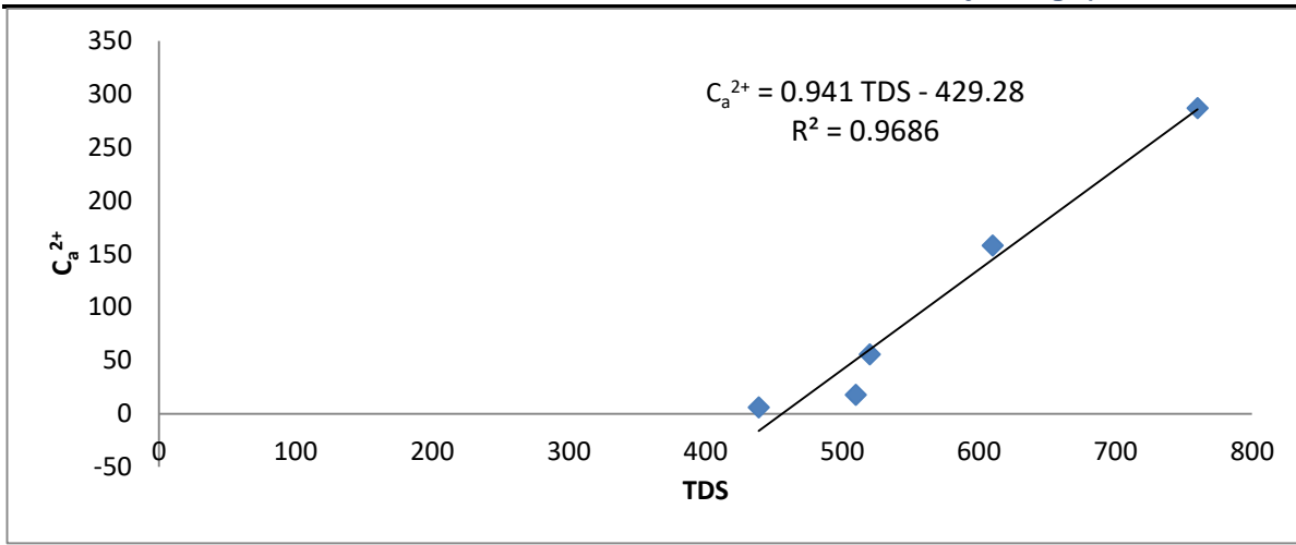
Fig 2: Correlation between TDS and C_a^{2+}
