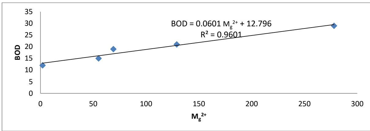
Fig 15: Correlation between M g 2+ and BOD
