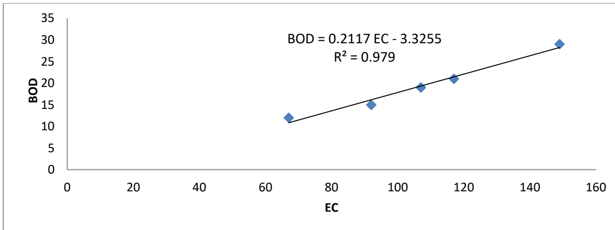
Fig 7: Correlation between EC and BOD
