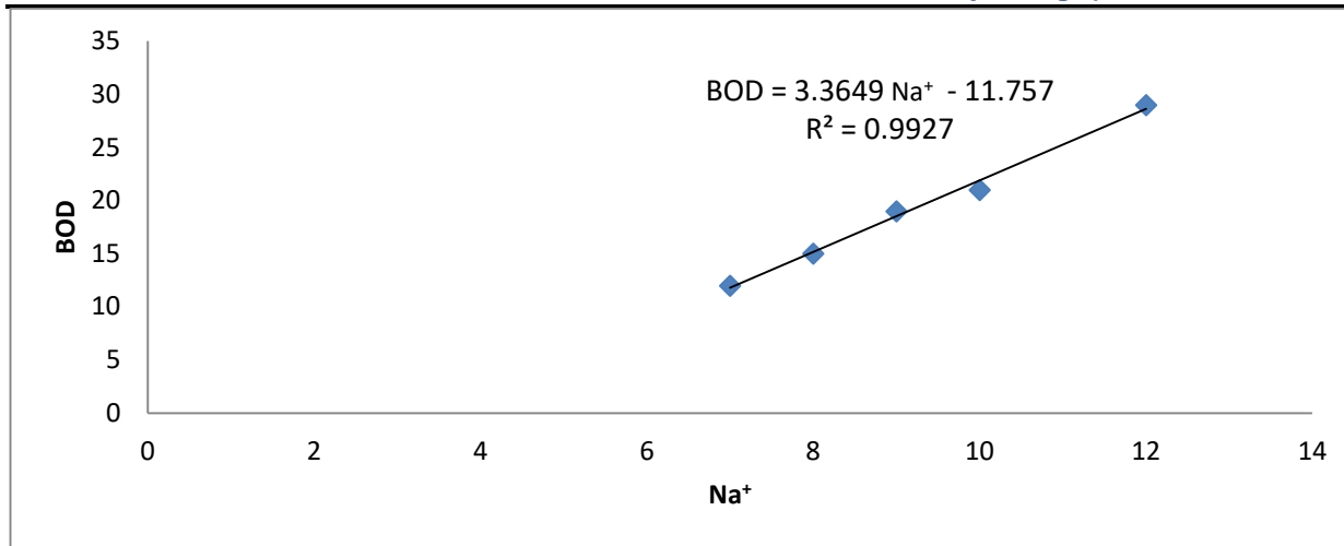
Fig 17: Correlation between Na + and BOD
