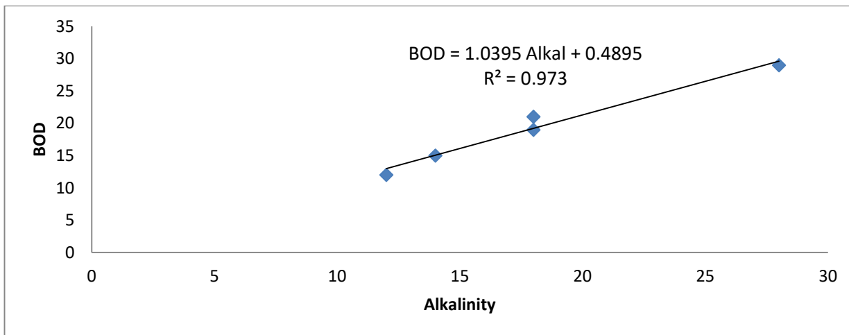
Fig 10: Correlation between Alkal and BOD
