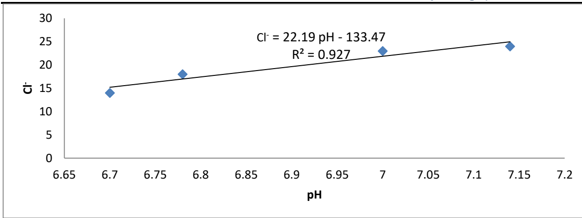
Fig 8: Correlation between pH and Cl -
