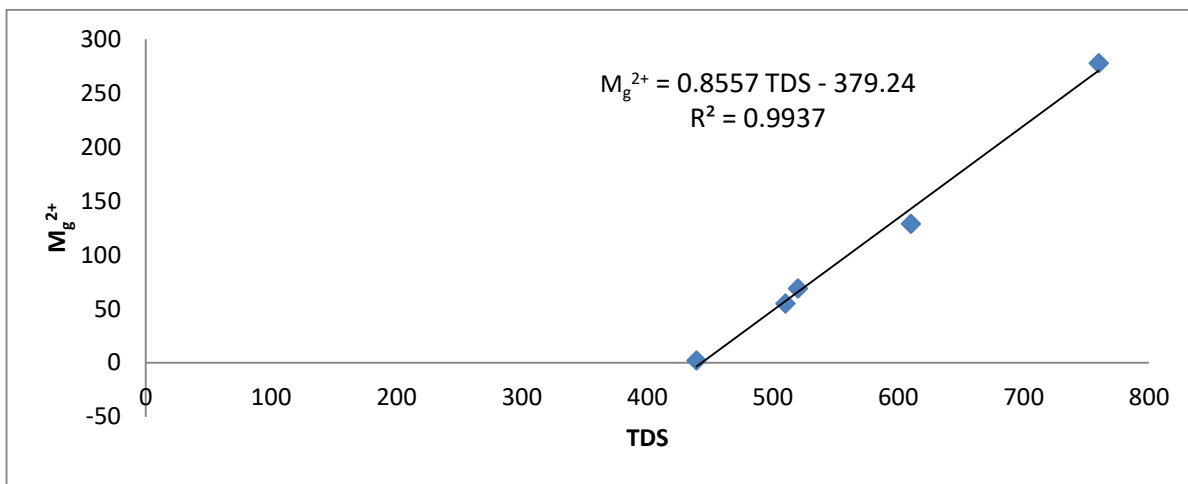
Fig 3: Correlation between TDS and M_g^{2+}
