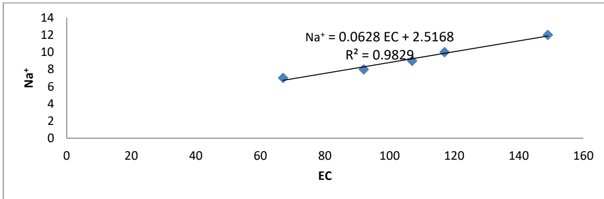
Fig 6: Correlation between EC and Na +
