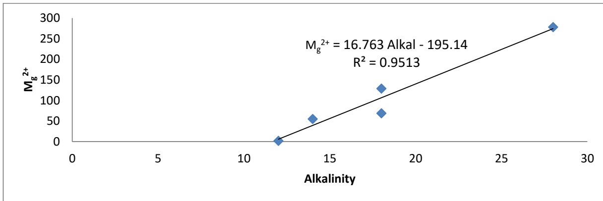
Fig 9: Correlation between Alkal and Mg 2+
