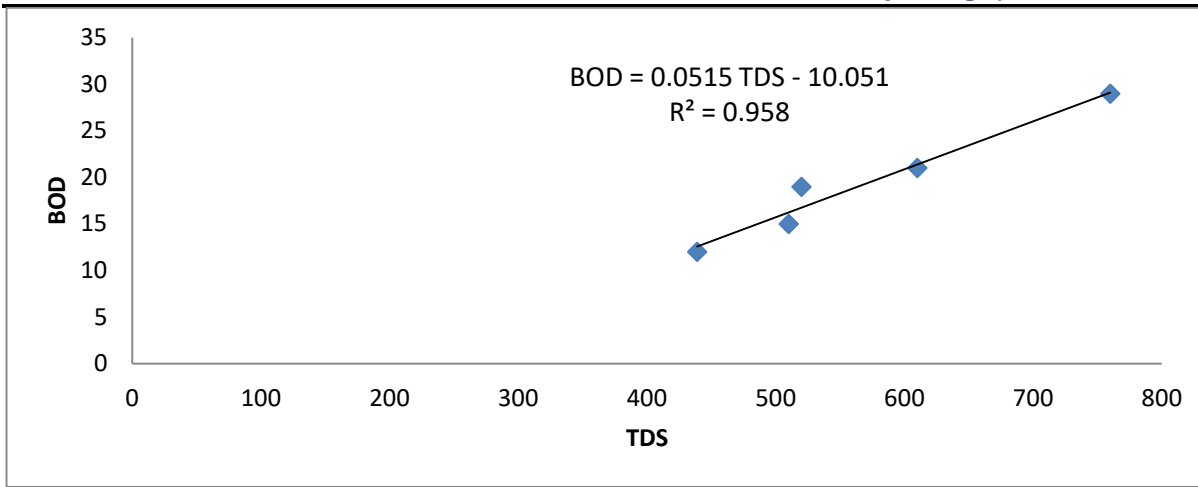
Fig 5: Correlation between TDS and BOD
