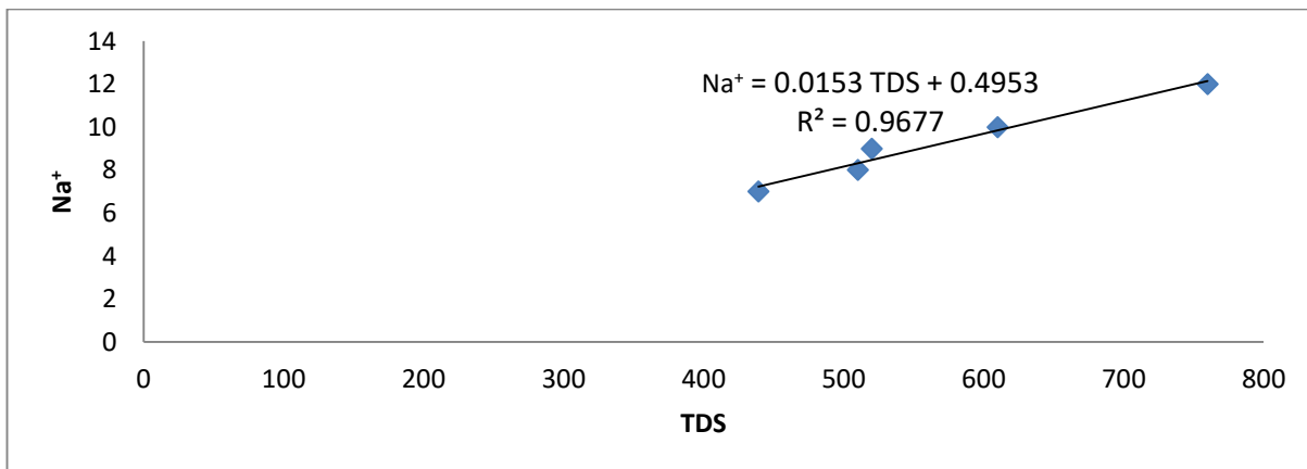
Fig 4: Correlation between TDS and Na^+
