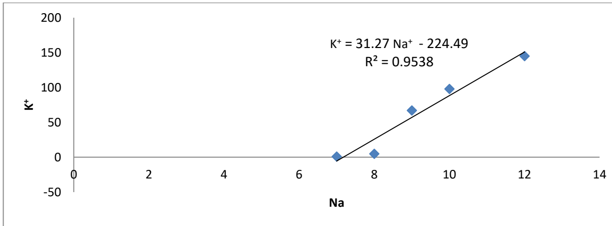
Fig 16: Correlation between Na + and K +
