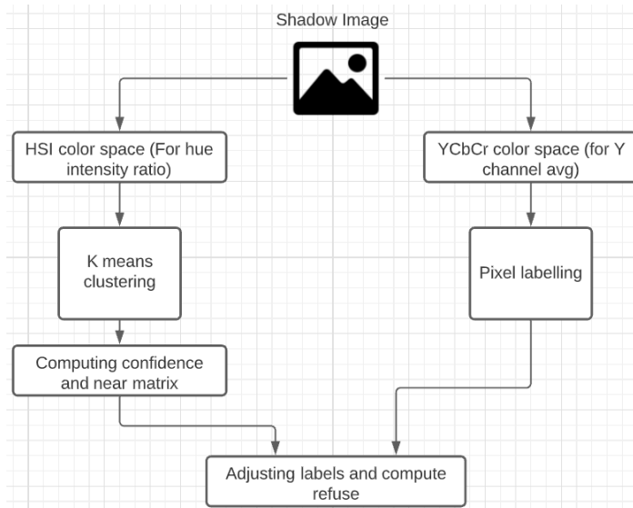
Fig 3.4. Shadow pixel detection
