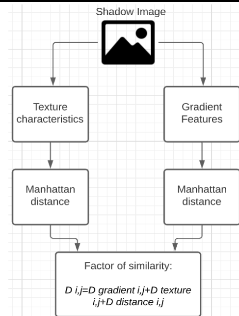
Fig 3.3. Area matching algorithm
